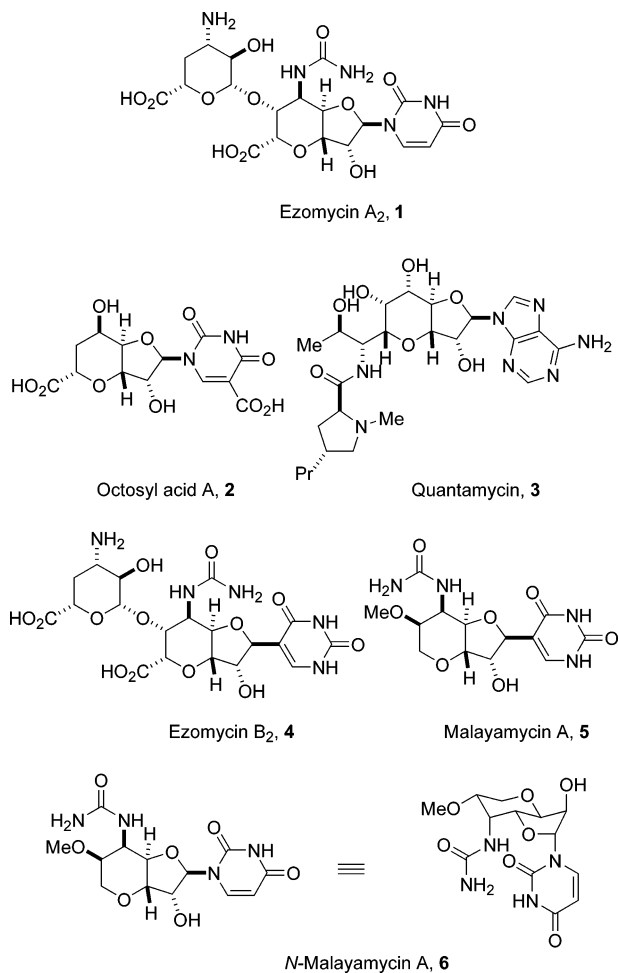
FIGURE 1. Structures of N - and C -bicyclic nucleosides.
