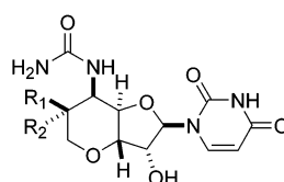
N -Malayamycin A and analogues; R 1 = OMe; R 2 = Me; R 1 = F; R 2 = H. R 1 = OMe; R 2 = H
