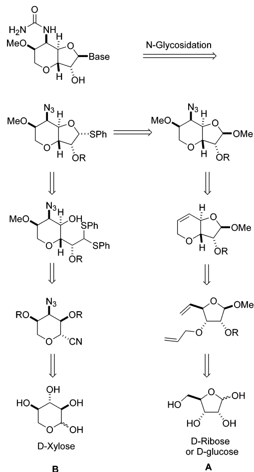
FIGURE 2. Disconnective analyses.
