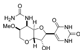
Malayamycin A
